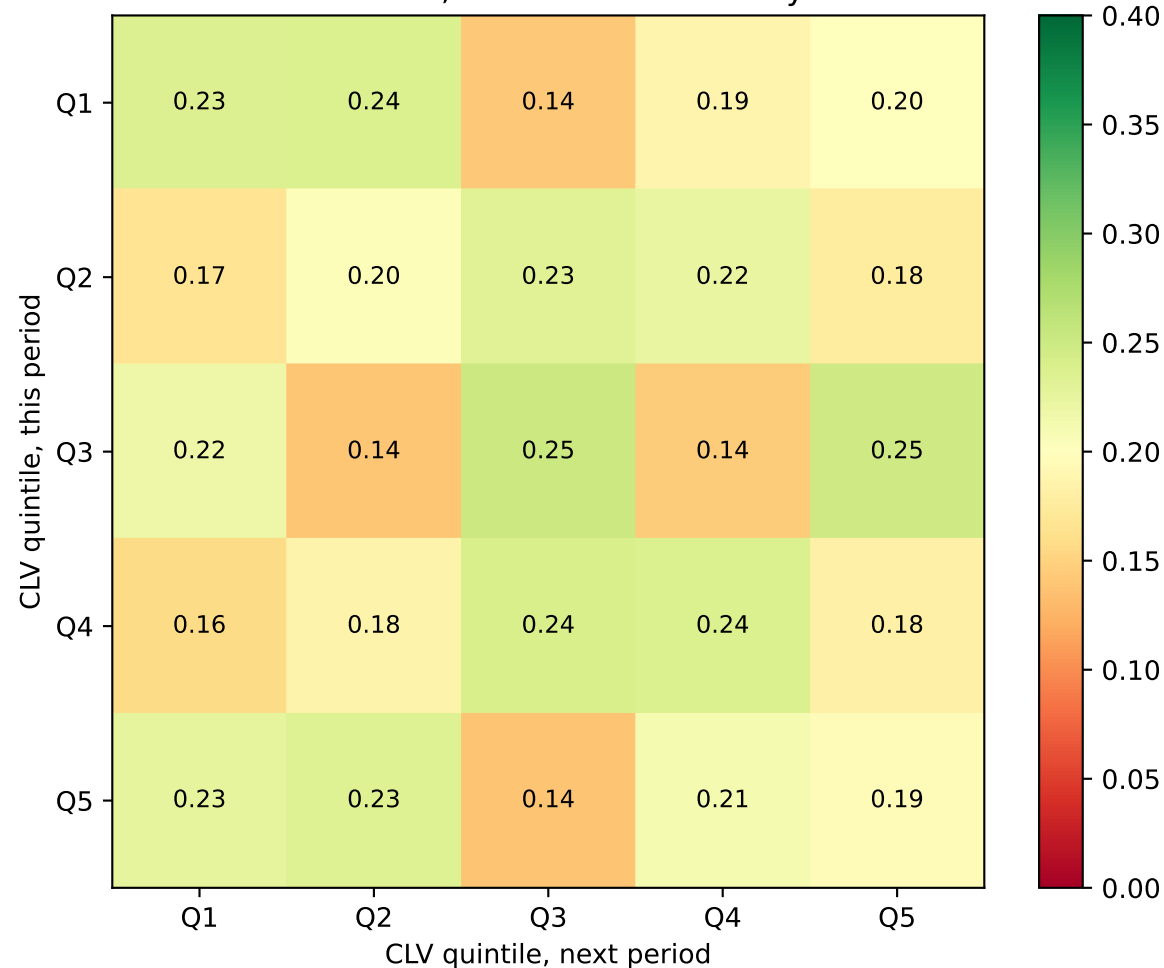
Quintile transition matrix (H2-2024->H1-2025) row-normalized; random = 0.20 everywhere
