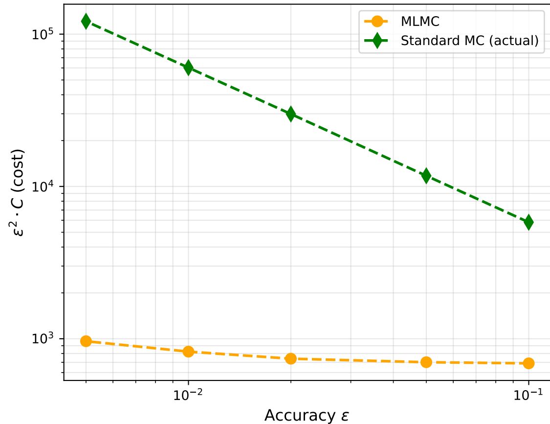
Complexity Comparison
