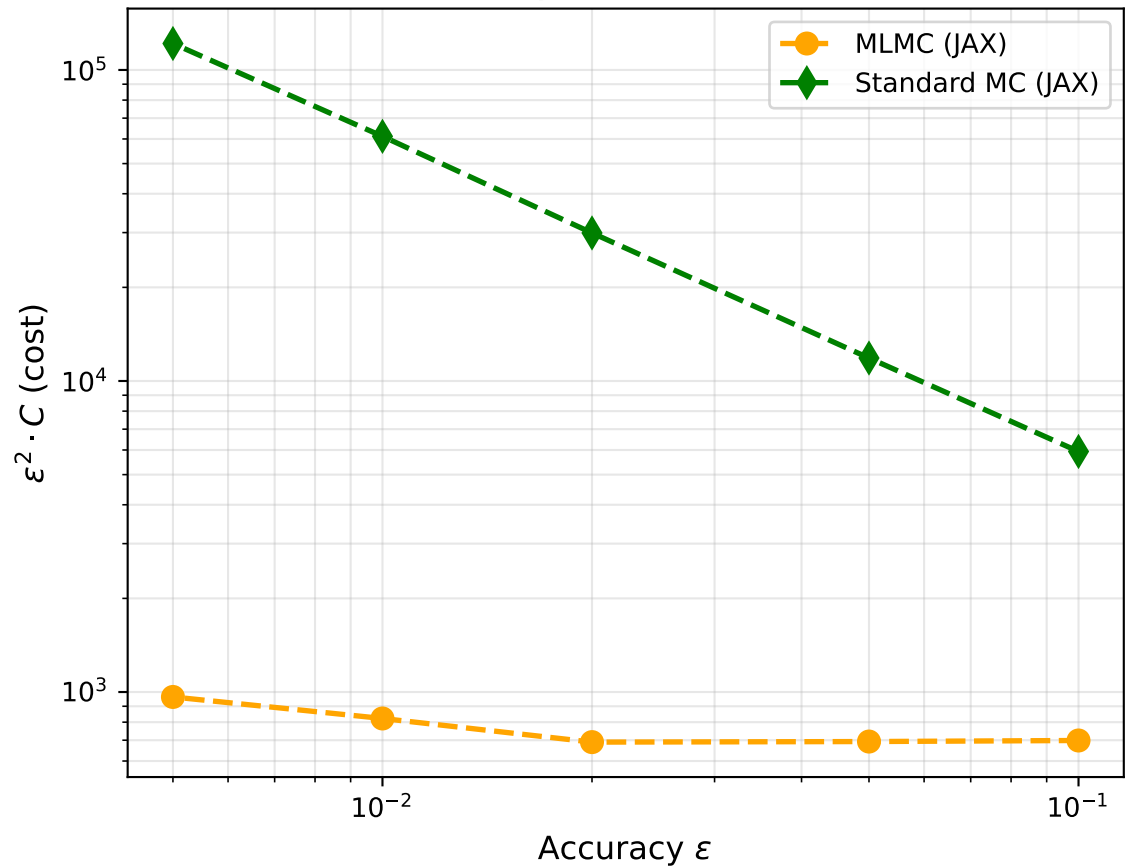
Complexity Comparison (JAX)
