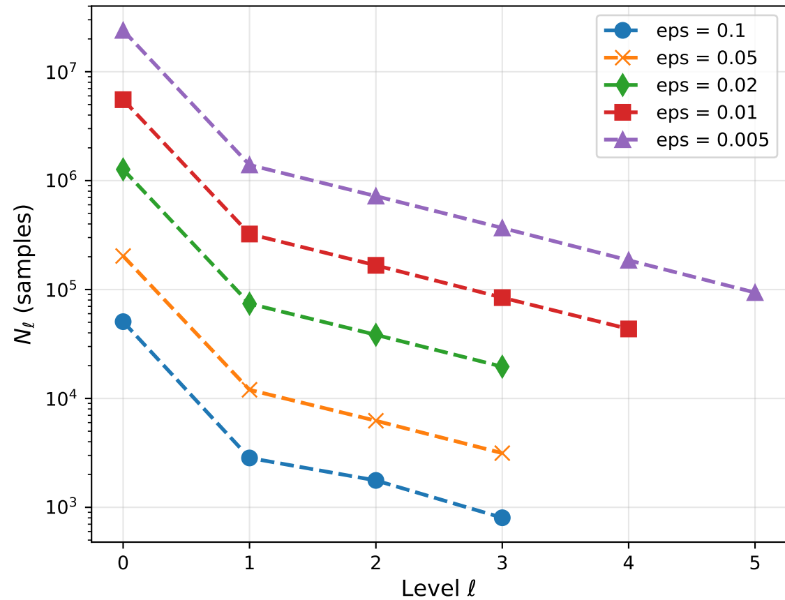
Optimal Sample Allocation (JAX)
