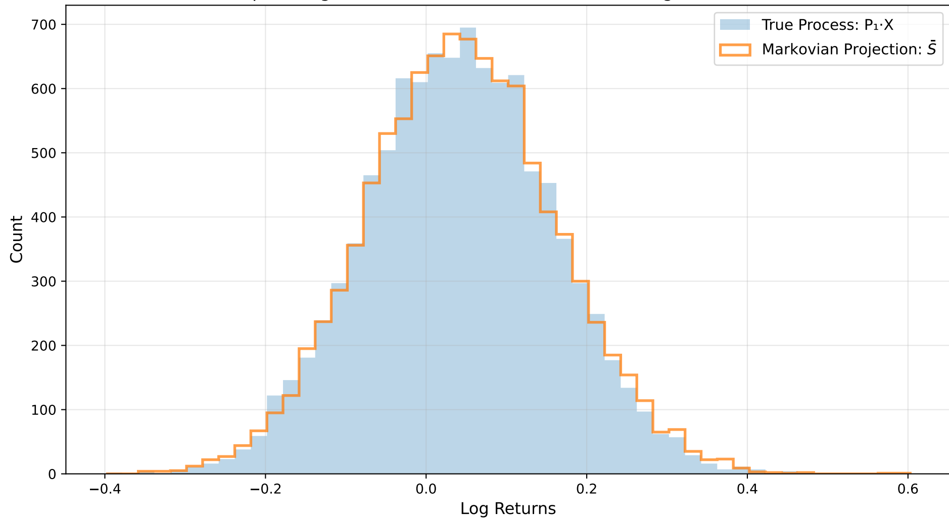
Terminal Distribution: True vs Projected Equal-weighted basket of 3 correlated stocks (Legendre basis)
