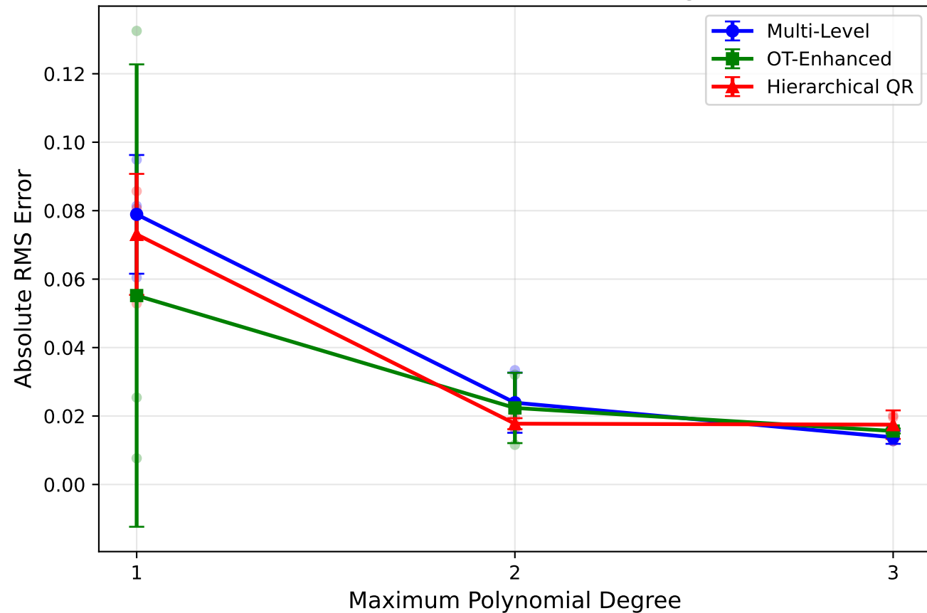
Absolute Error: ML Methods vs Single-Level
