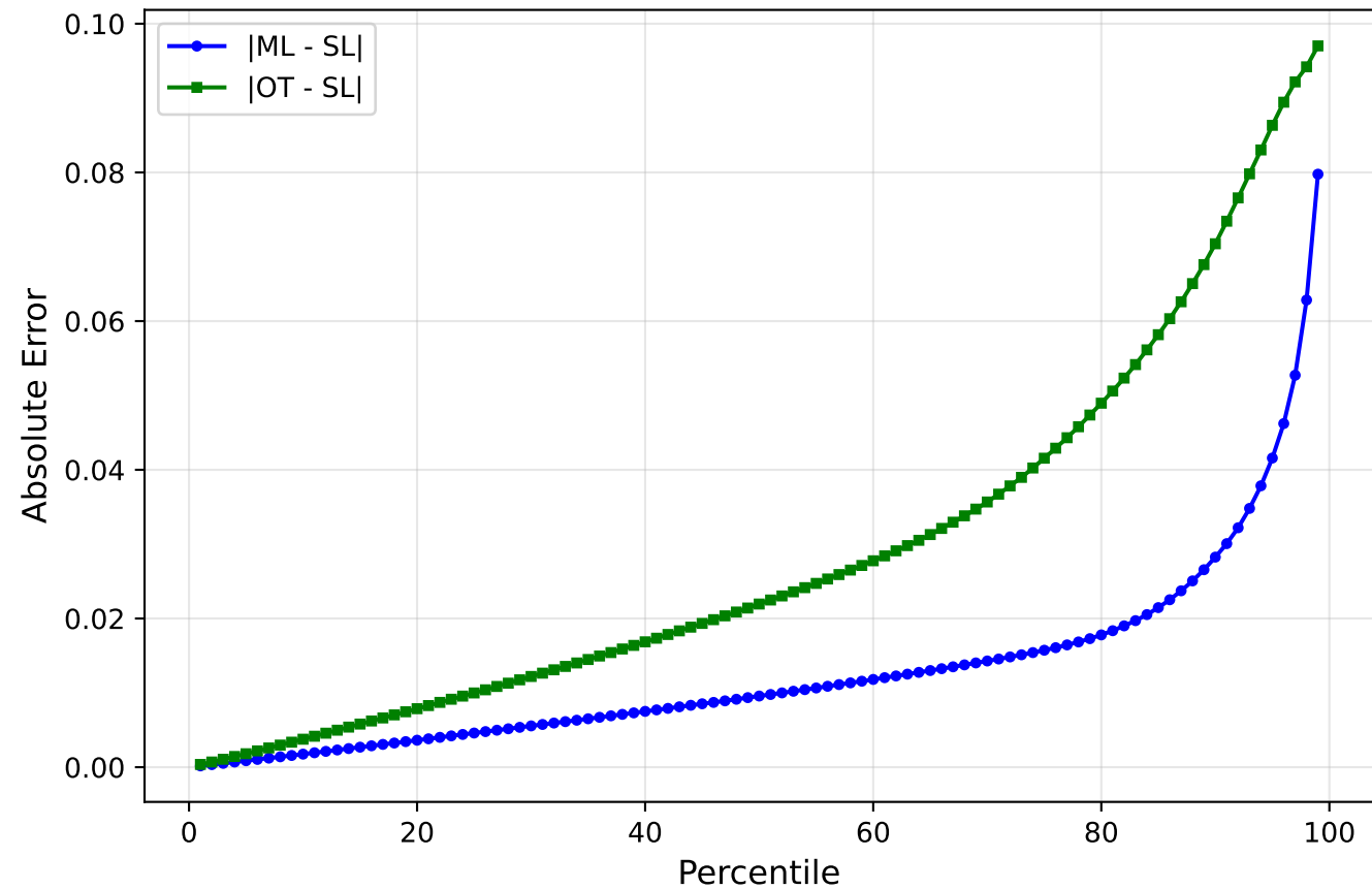
Error Percentiles
