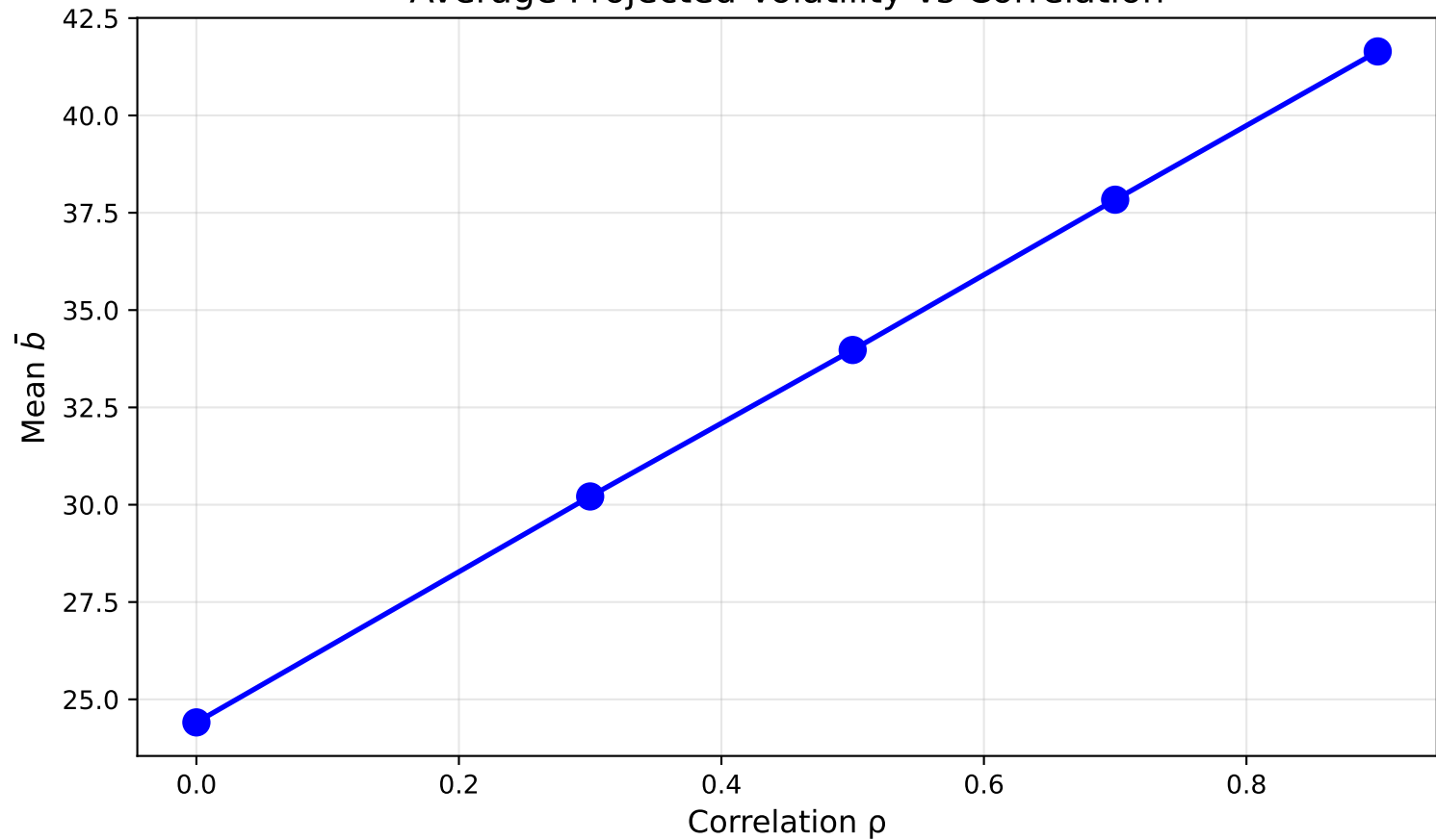
Average Projected Volatility vs Correlation
