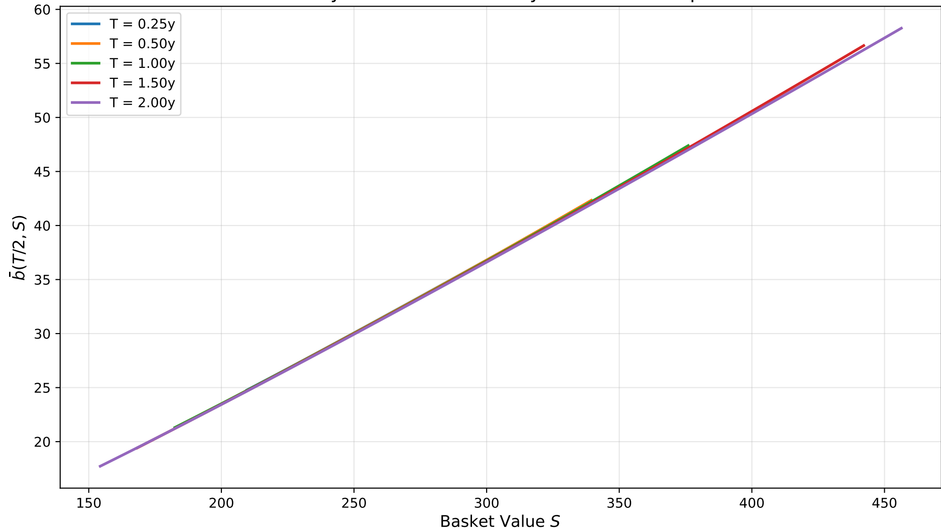
Volatility Slice at Mid-Maturity for Different Expiries
