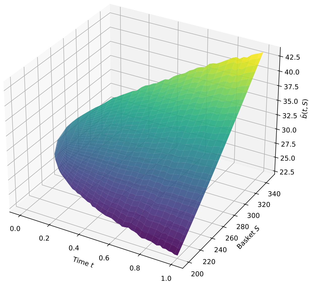
OT-Enhanced MLMC
