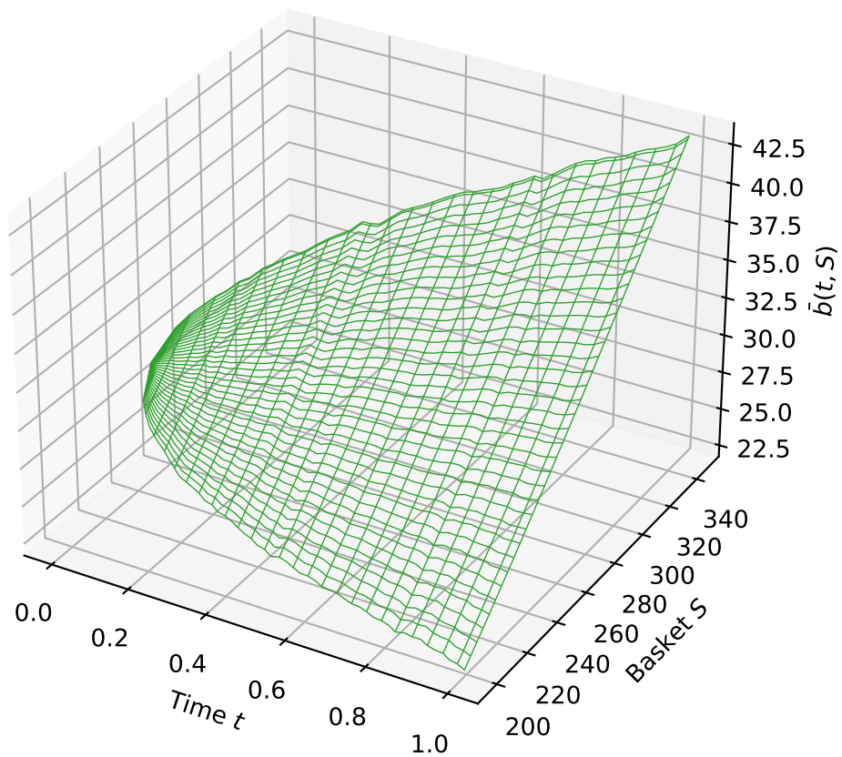
OT-MLMC Volatility Surface (max degree = 2)
