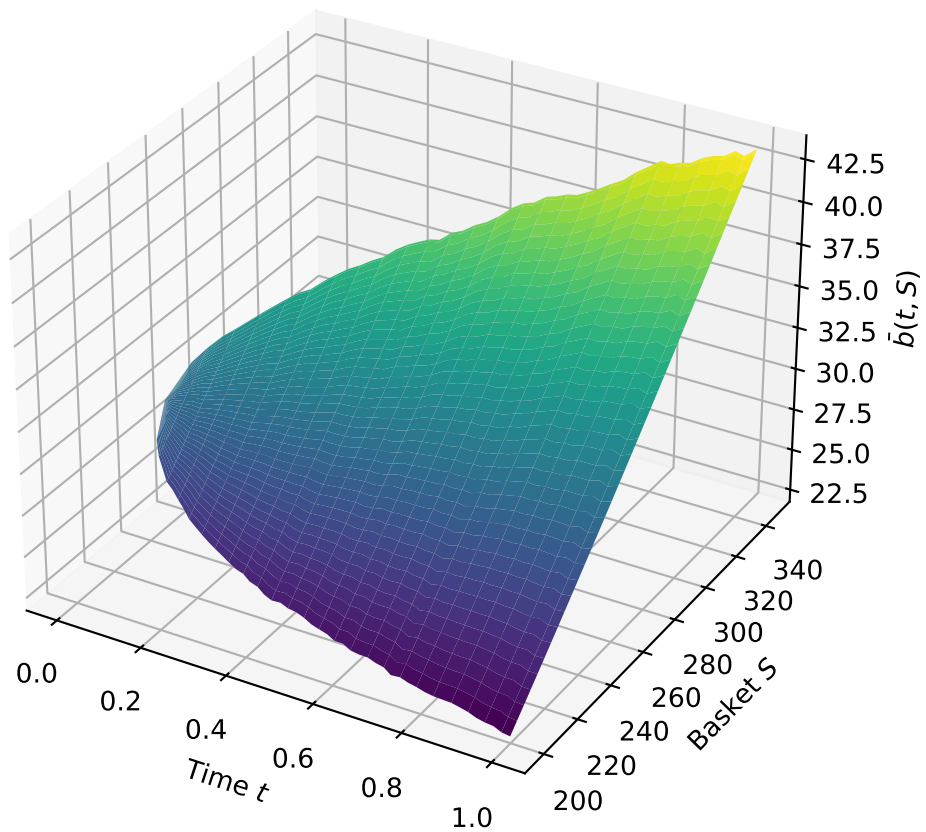
Projected Volatility Surface (max degree = 3)
