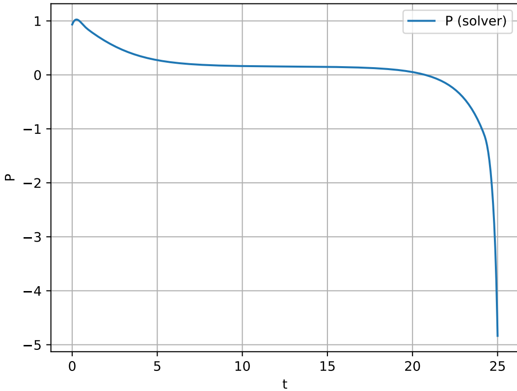
Example 5: Costate P(t)
