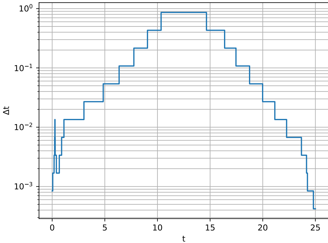
Time mesh: \Delta t(t) (step plot)
