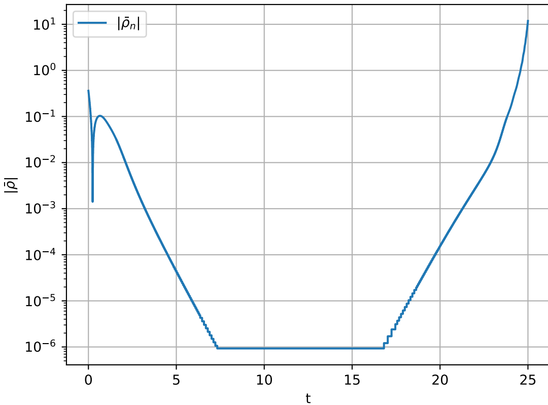
Example 5: density-like term \bar{\rho}_n
