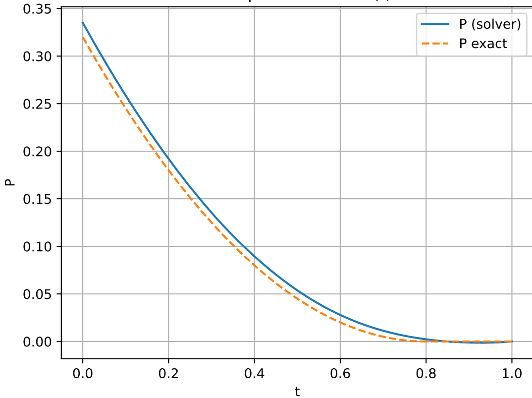
Example 4: Costate P(t)
