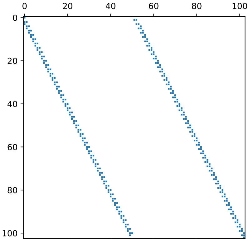
Jacobian pattern (current z-order: x-block then p-block)
