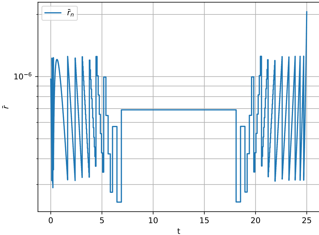
Example 5: time error indicator \bar{r}_n = |\bar{\rho}_n| \Delta t_n^2
