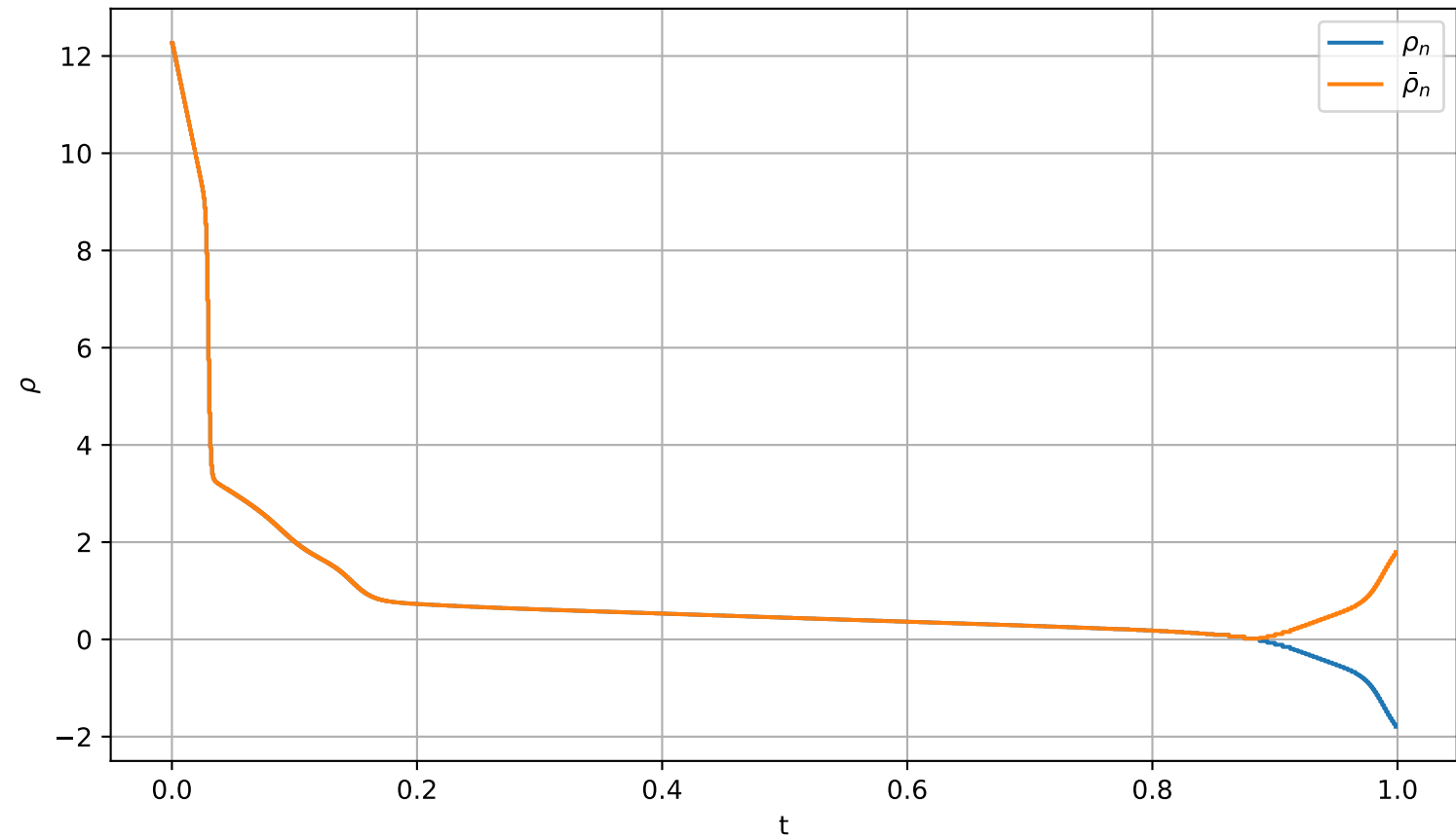
Error density: \rho_n , \bar{\rho}_n
