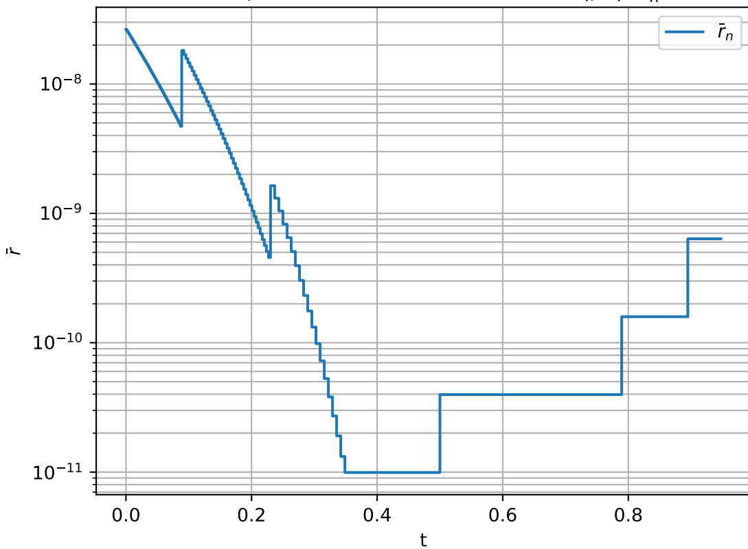
Example 6: time error indicator \bar{r}_n = |\bar{\rho}_n| \Delta t_n^2
