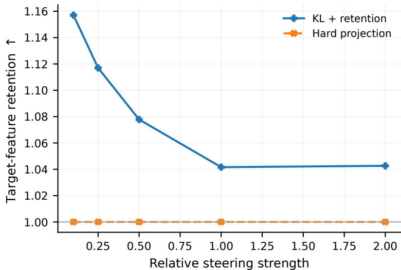
Independent sentiment direction
