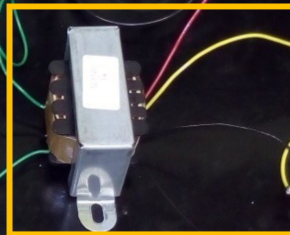
Grid voltage Transformer 127V to 12V
