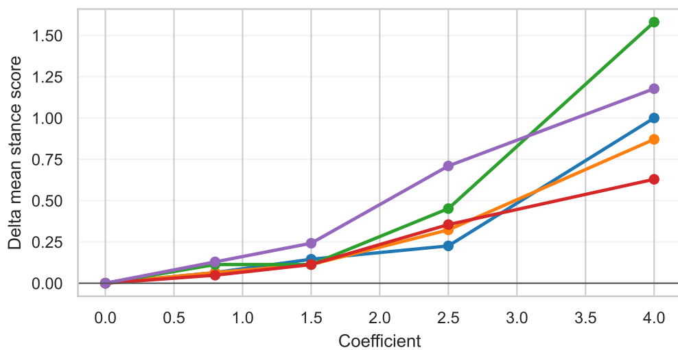
Llama-3-8B-Instruct left steering
