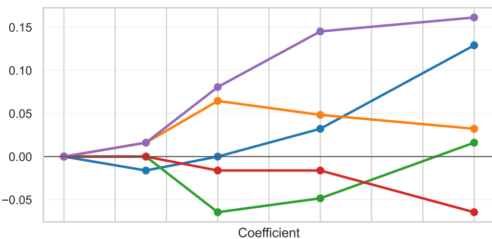
Qwen2.5-7B-Instruct left steering
