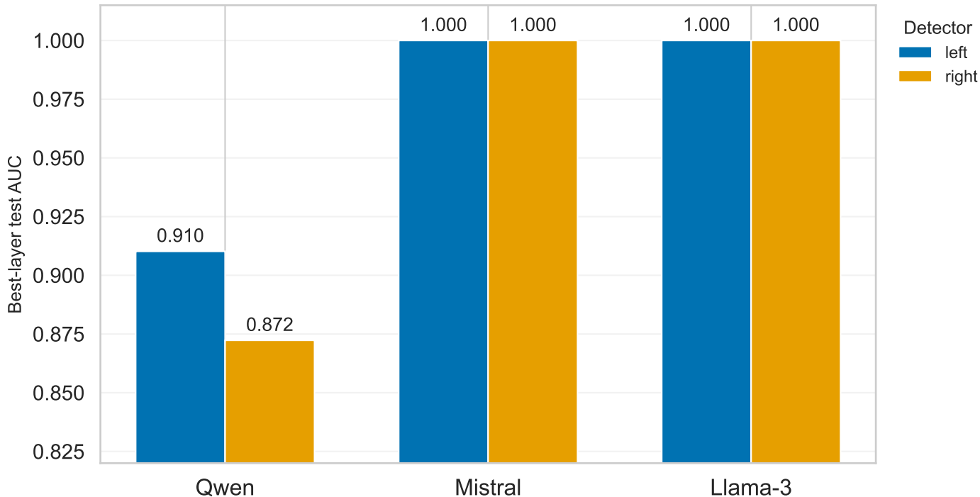
Best-layer test AUC by model and detector
