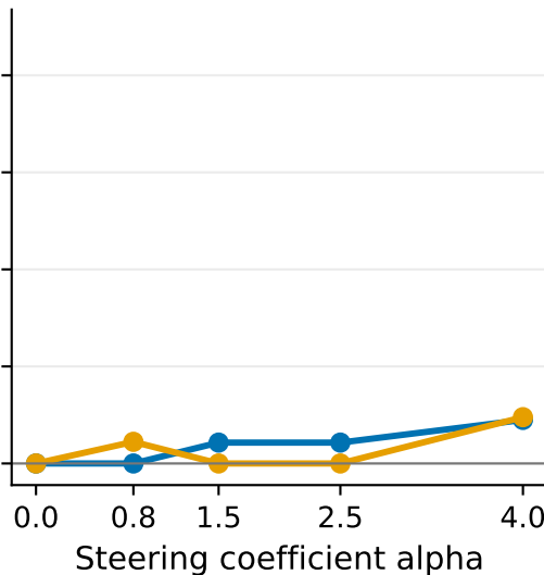
Mistral
