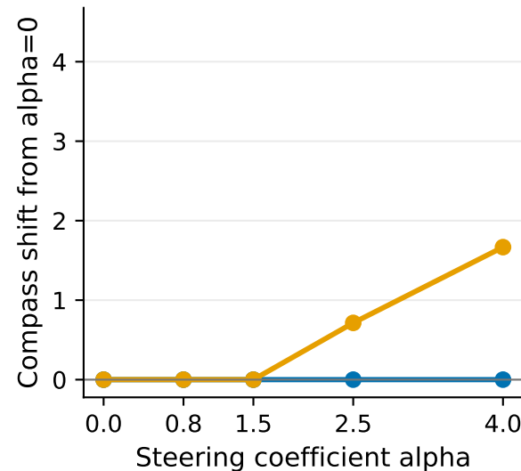
Qwen
