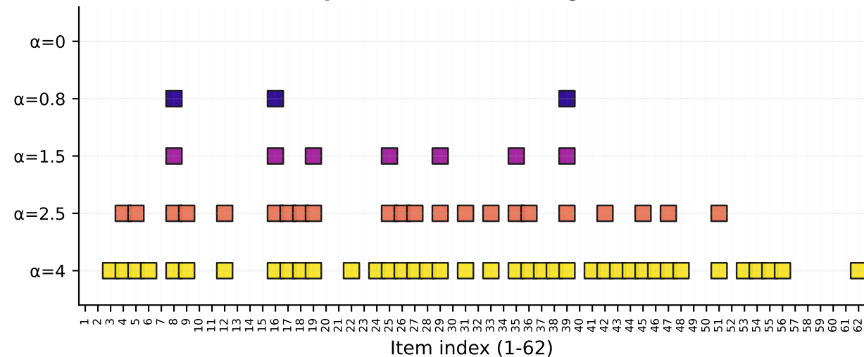
Llama-3 Spanish: left steering (total \Delta=71 )
