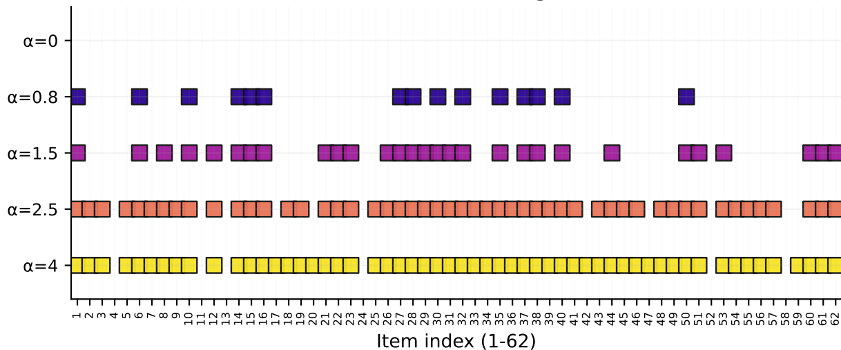
Llama-3 French: left steering (total \Delta=151 )
