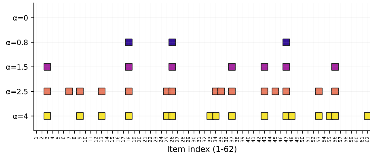
Qwen German: left steering (total \Delta=41 )
