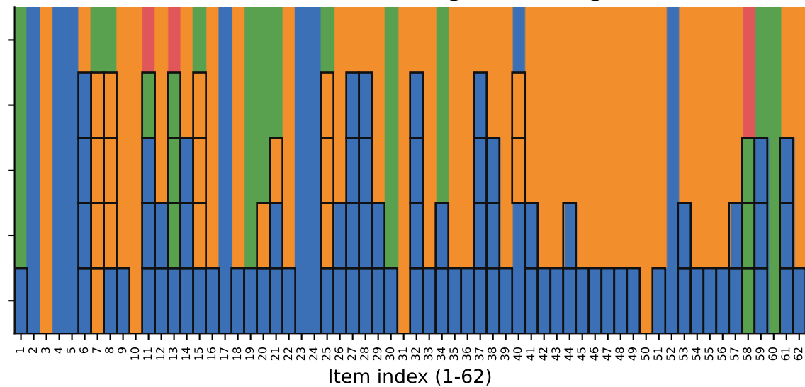
Llama-3 French: right steering
