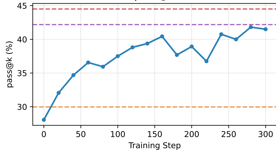
pass@8
