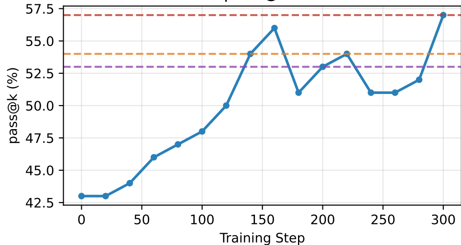
pass@16
