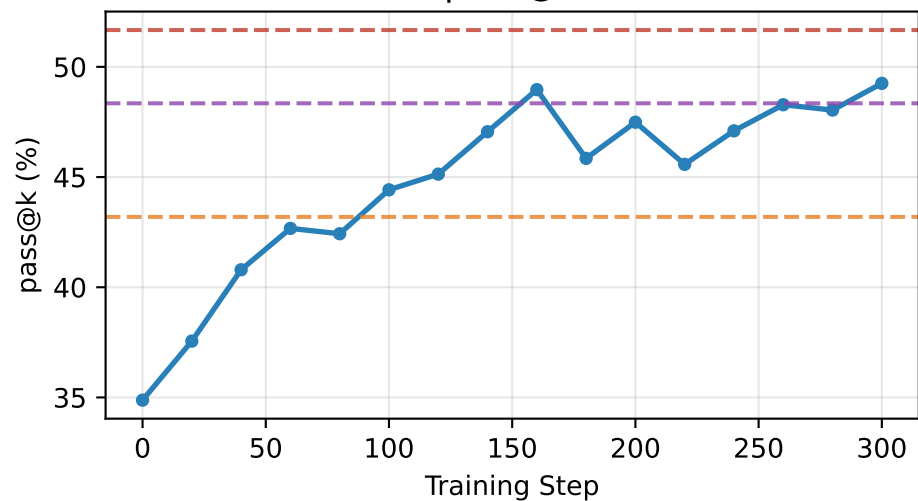
pass@16
