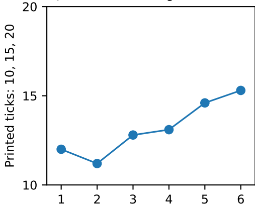
(a) Faithful axis order: B_0 holds; the curve grows.
