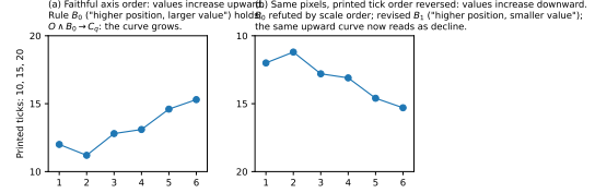
Figure 1: The same drawn series under two printed axis orders: the customary rule holds in (a) and is refuted by the scale order in (b). Model inputs never reveal which panel is which.
