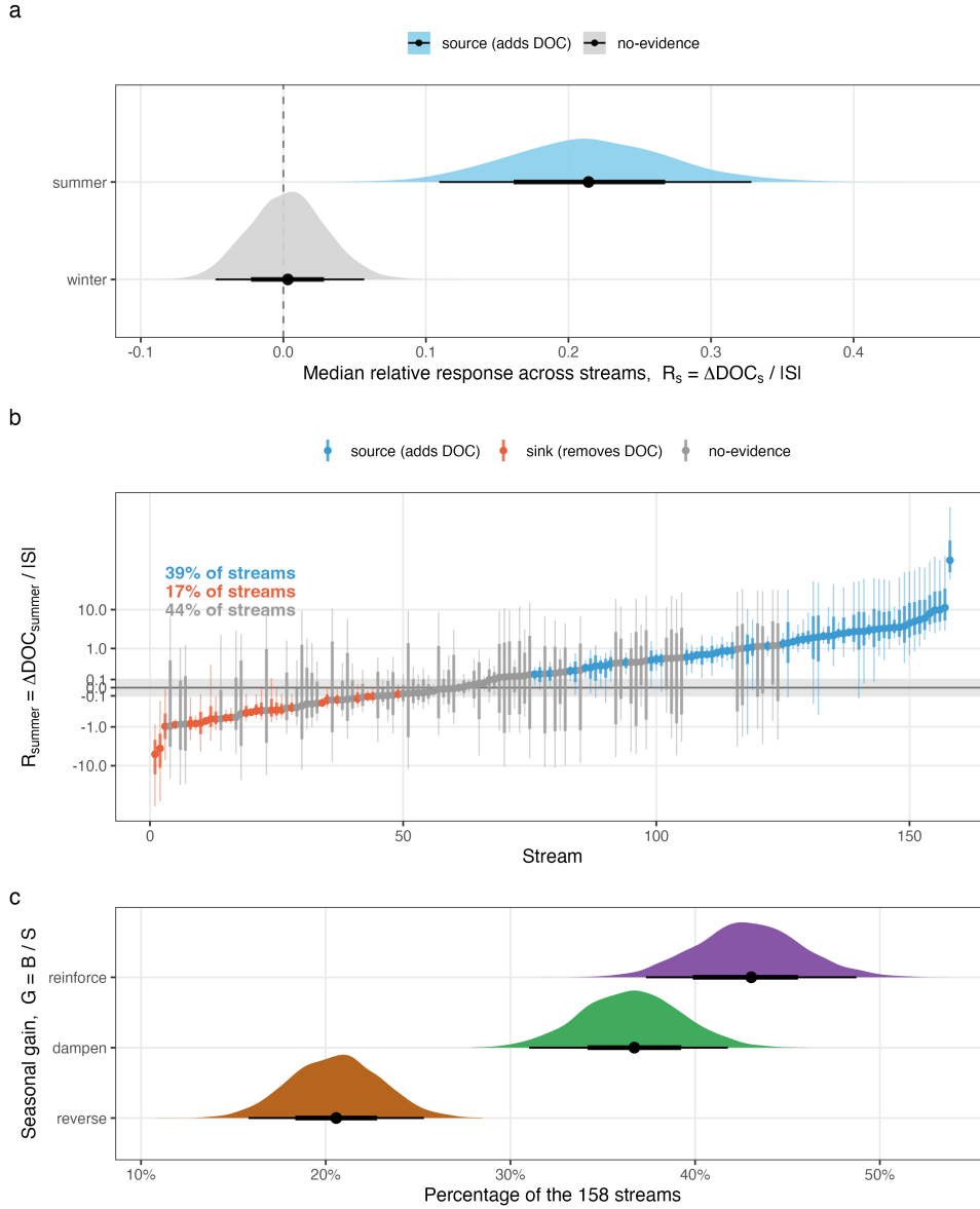
Fig. 3 a) Posterior distribution of the median relative response R_s = \Delta DOC_s / |S| across the 158 streams, in winter and summer; point: posterior median, bars: 66% and 95% credible intervals; dashed line: no response; skyblue: beaver-engineering adds DOC (posterior probability > 90%), grey: no-evidence. b) Relative response of each stream in summer: posterior median with 66% (thick) and 95% (thin) credible intervals, streams ranked by their median; the grey band marks |R_{summer}| < 0.1 ; the vertical axis is linear between -0.1 and 0.1 and logarithmic beyond. Skyblue: source (adds DOC), coral: sink (removes DOC), grey: no-evidence (same threshold as in a); percentages give the share of the 158 streams in each colour. c) Posterior share of the 158 streams whose seasonal gain G = B/S reinforces ( G > 0 ), dampens ( -1 < G < 0 ) or reverses ( G < -1 ) the inherited seasonal contrast; each stream is classified on every posterior draw, so each distribution is the posterior uncertainty of the share itself; point: posterior median, bars: 66% and 95% credible intervals.
