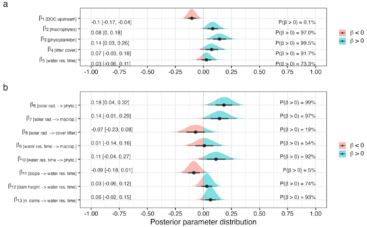
Figure S5: Posterior parameters distributions of the fitted SCM. Median shown with point; 66% and 95% credible intervals shown with black bars. Parameters that have more than 90% probability mass on either side of zero are considered to have a positive or negative influence on the response variable. a) The direct effects on \Delta\text{DOC} b) The indirect effects on \Delta\text{DOC} .
