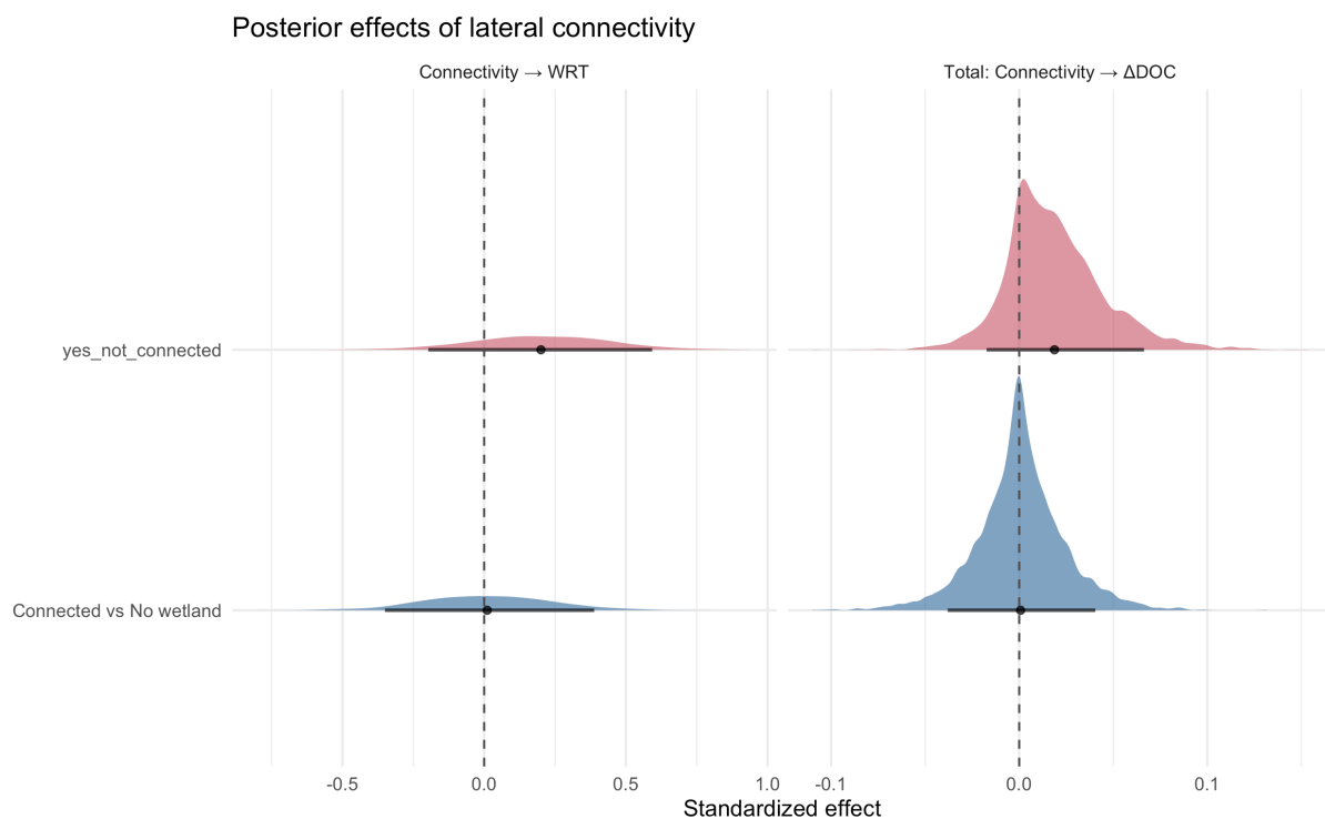
Figure S9: Posterior effects of lateral stream–wetland connectivity (relative to sites without wetland) on water residence time (left) and the total mediated effect on \Delta\text{DOC} (right), controlling for beaver-dam variables, channel gradient and solar radiation. Points show posterior means; thick and thin bars show the 66% and 90% credible intervals. The dashed line marks zero.
