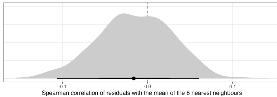
Figure S14: Spatial autocorrelation of the residuals of downstream DOC. For each posterior draw, the Spearman correlation between each sampling's residual (observed minus expected downstream DOC) and the mean residual of its 8 nearest neighbouring samplings, using the stream coordinates; point: median, bars: 66% and 95% credible intervals; dashed line: no spatial autocorrelation.
