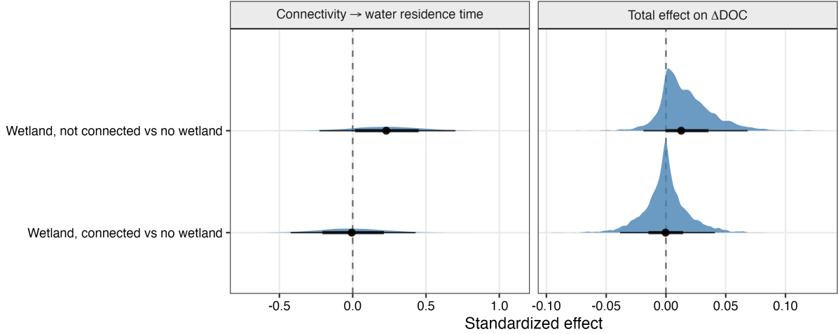
Figure S8: Posterior effects of lateral stream–wetland connectivity (relative to sites without wetland) on water residence time (left) and the total mediated effect on \Delta\text{DOC} (right), controlling for beaver-dam variables, channel gradient and solar radiation. Points: posterior medians; thick and thin bars: 66% and 95% credible intervals. The dashed line marks zero.
