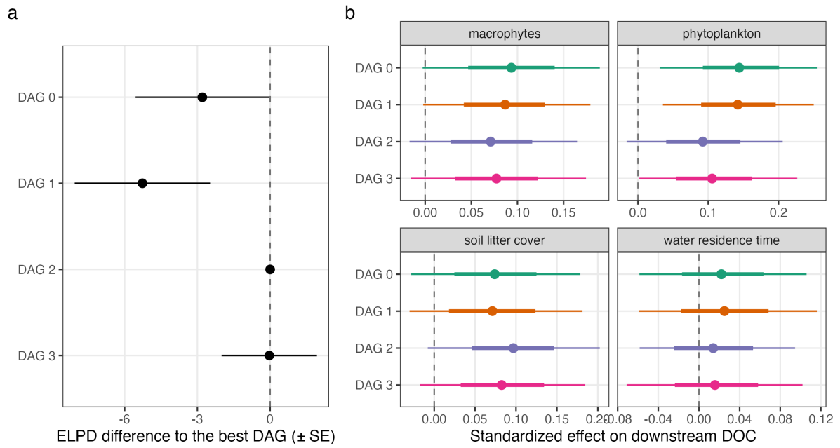
Figure S10: The four causal structures fitted as multivariate Bayesian models. a) Out-of-sample fit for downstream DOC by Pareto-smoothed importance-sampling leave-one-out cross-validation (PSIS-LOO): expected log predictive density relative to the best-fitting structure (0 = best), with standard error; a difference smaller than about 4 is not meaningful. b) The mediator effects on downstream DOC under each structure: posterior median with 66% and 95% credible intervals.
