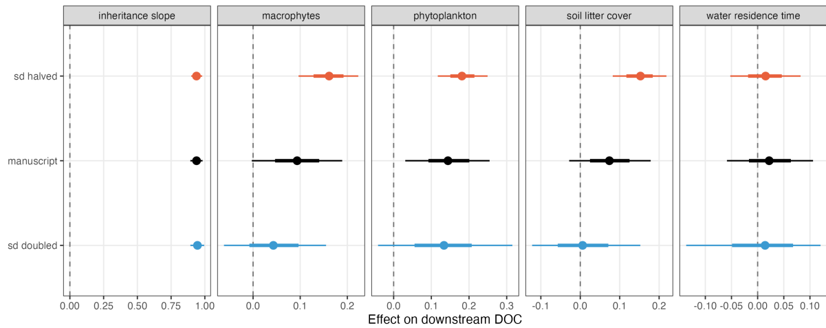
Figure S13: Prior sensitivity. Mediator effects on downstream DOC when the standard deviation of every informative prior is halved, kept as in the manuscript, or doubled; posterior median with 66% and 95% credible intervals. A path whose estimate follows the prior scale is prior-driven; a path that stays put is data-driven.
