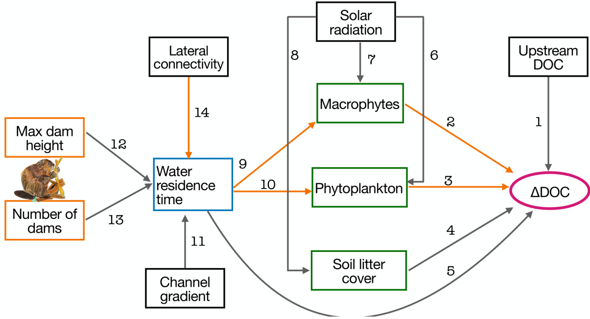
Figure S7: Extended directed acyclic graph (DAG) of the alternative SCM. It is identical to the main SCM (Figure S1) except for the additional causal path 14, connecting lateral stream–wetland connectivity to water residence time. Orange edges mark the open front-door paths through which the total causal effect of lateral connectivity flows to \Delta\text{DOC} (paths 14 \rightarrow 9 \rightarrow 2, 14 \rightarrow 10 \rightarrow 3, and 14 \rightarrow 5).
