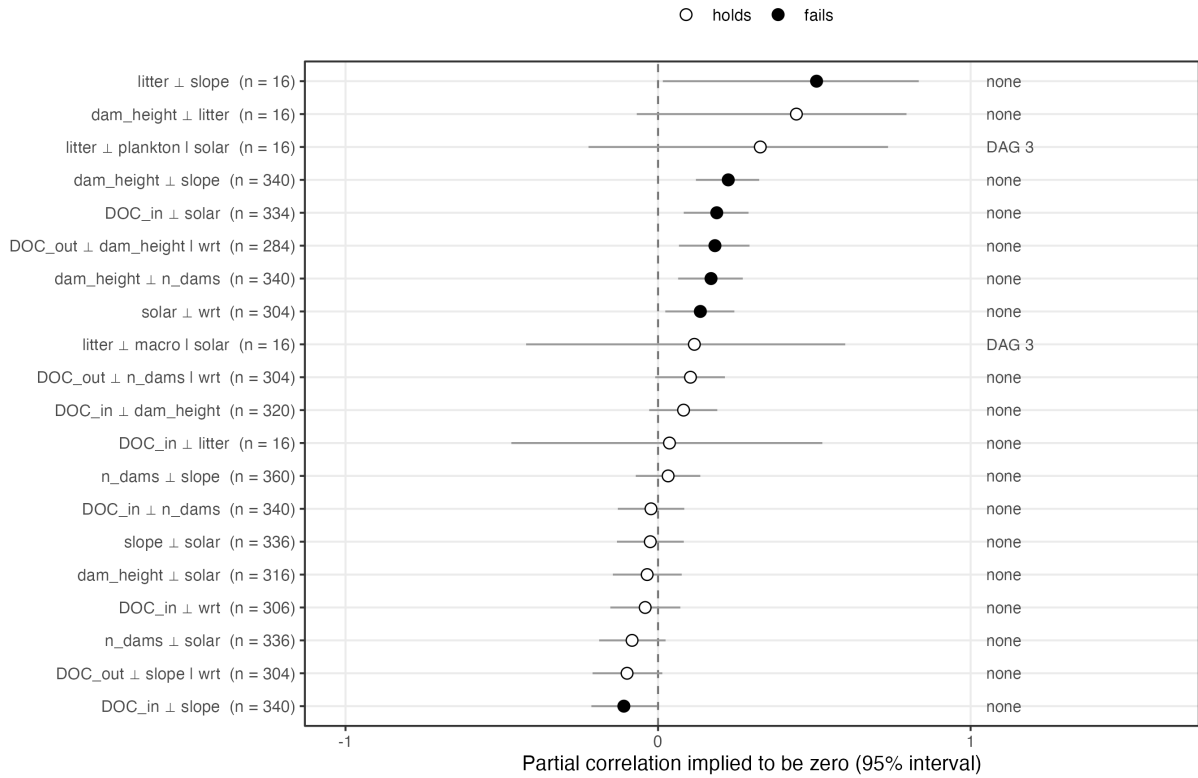
Figure S9: Conditional independencies implied by the reported structural causal model (DAG 0), tested on the data. Each row is one independence the model implies; the point is the partial correlation on the rows complete for the variables involved, with its 95% interval and the number of samplings used. Filled points: the interval excludes zero (the independence fails). The right-hand label names the alternative structure(s) that would drop that independence, i.e. that a failure would support.
