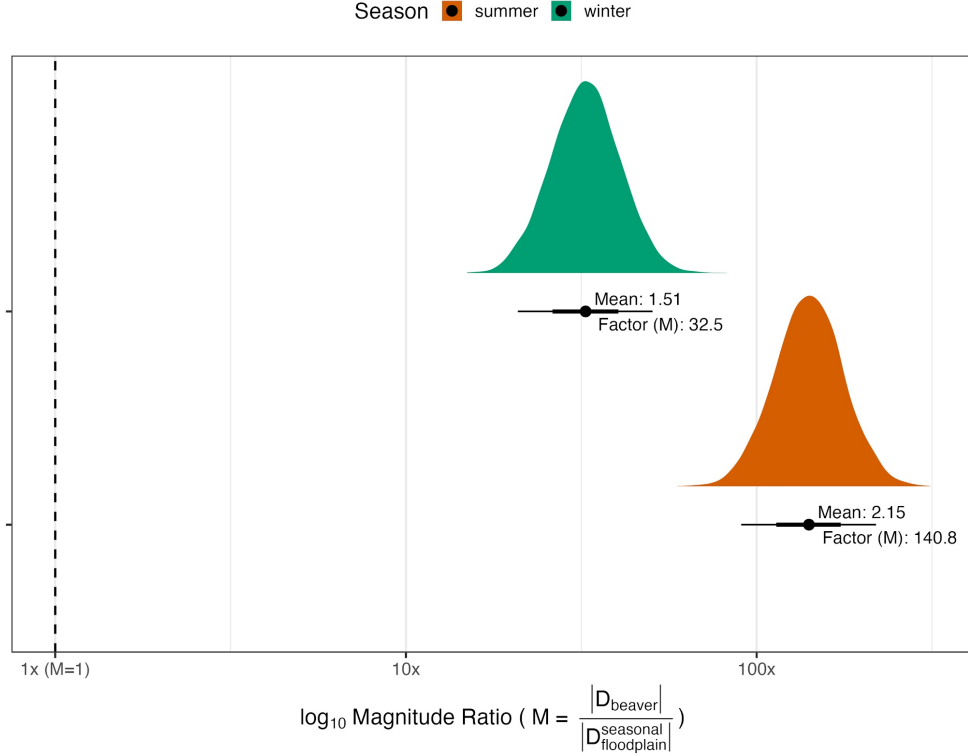
Fig. 3 Posterior distribution of the beaver amplification factor M , comparing the beaver mediated change in DOC to the seasonal floodplain-scale DOC change per unit area. The vertical dashed line at 0 represents the line of equivalence, where the magnitudes are equal. The central dot marks the posterior mean. The thick inner segment shows the 66% credible interval, and the thinner outer segment shows the 95% CI. Green represents winter, and orange represents summer.
