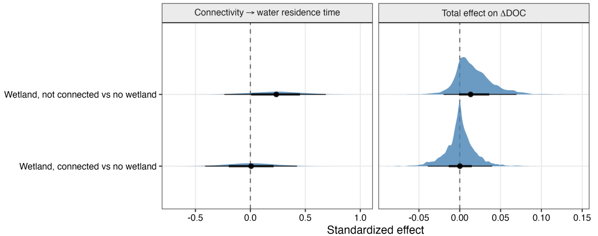
Figure S9: Posterior effects of lateral stream–wetland connectivity (relative to sites without wetland) on water residence time (left) and the total mediated effect on \Delta\text{DOC} (right), controlling for beaver-dam variables, channel gradient and solar radiation. Points: posterior medians; thick and thin bars: 66% and 95% credible intervals. The dashed line marks zero.
