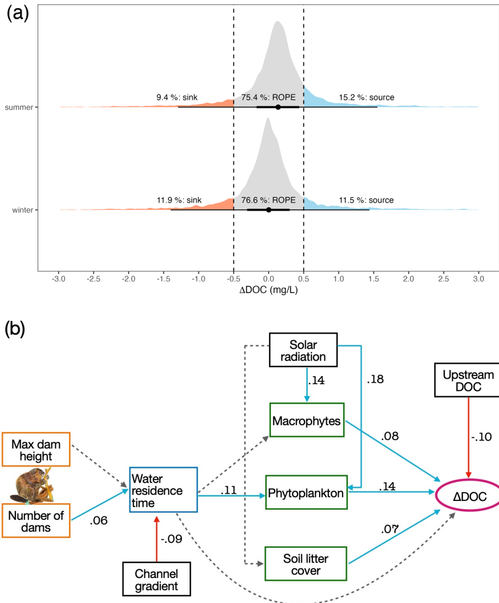
Fig. 1 a) Posterior predictive distribution of \Delta\text{DOC} for a single sampling of a beaver-engineered stream, in summer and winter (measurement-error model on raw upstream and downstream DOC concentrations). The orange shaded area represents the posterior predictive probability that a single sampling shows a DOC sink response; the light blue shaded area the probability of a DOC source response. The grey shaded area represents the Region Of Practical Equivalence (ROPE) and it defines an interval around zero where effects are too small to be of practical importance. The central dot indicates the median of the distribution, while the thick and thin horizontal lines represent the 66% and 95% intervals. b) Drivers of beaver-mediated DOC change. Solid edges (red = negative, blue = positive) represent 90% probability evidence of causal effects; dashed edges represent inconclusive evidence. Standardized average effects are shown. Full posterior parameter distributions in Appendix S1: Figure S4. Beaver illustration credits to © Sarah Edmonds Illustration.
