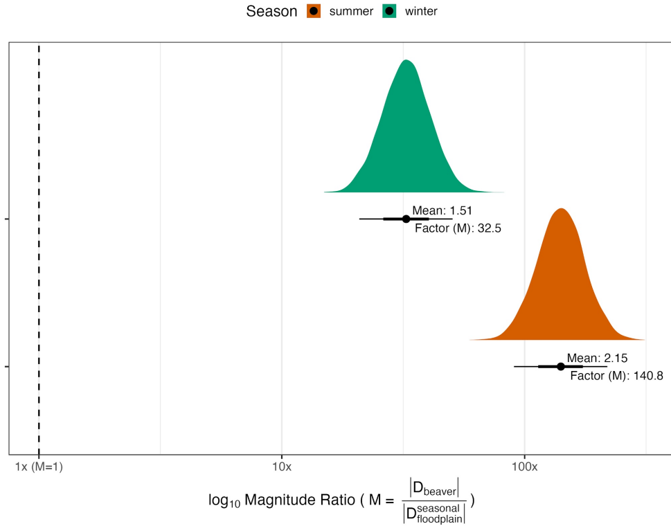
Fig. 2 Posterior distribution of the beaver amplification factor M, comparing the beaver mediated change in DOC to the seasonal floodplain-scale DOC change per unit area. The vertical dashed line at 0 represents the line of equivalence, where the magnitudes are equal. The central dot marks the posterior mean. The thick inner segment shows the 66% credible interval, and the thinner outer segment shows the 95% CI. Green represents winter, and orange represents summer.
