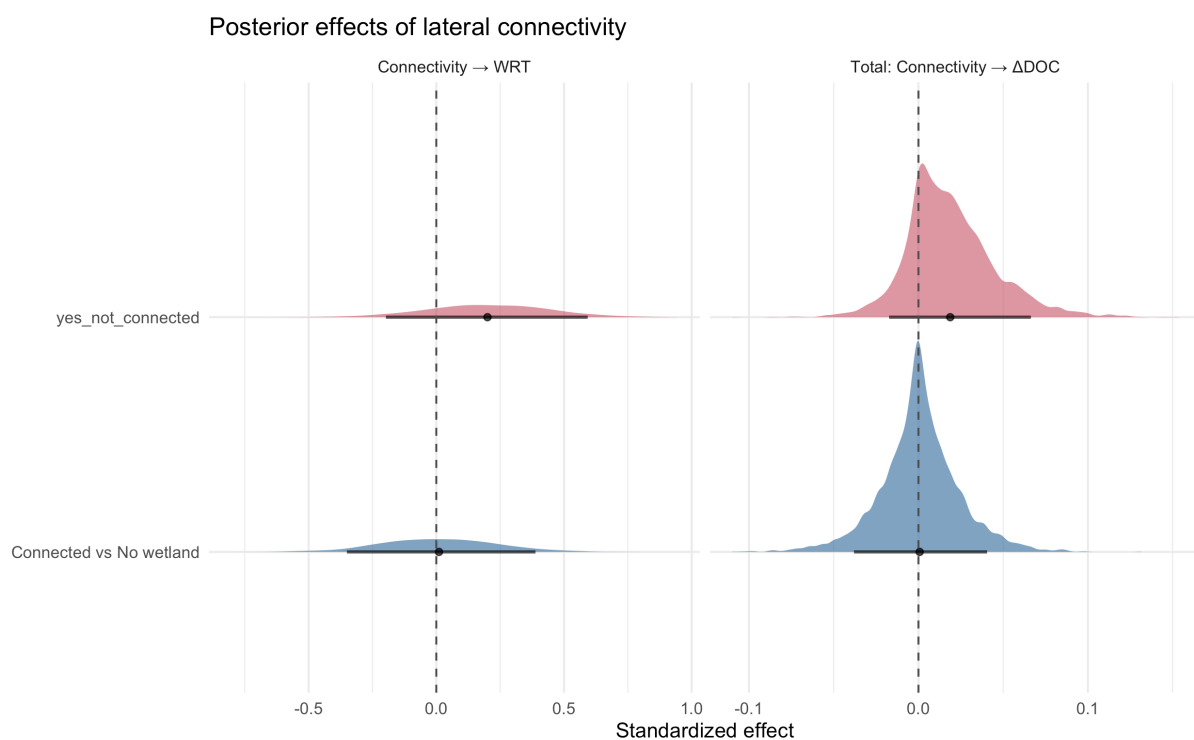
Figure S8: Posterior effects of lateral stream–wetland connectivity (relative to sites without wetland) on water residence time (left) and the total mediated effect on \Delta DOC (right), controlling for beaver-dam variables, channel gradient and solar radiation. Points show posterior means; thick and thin bars show the 66% and 90% credible intervals. The dashed line marks zero.
