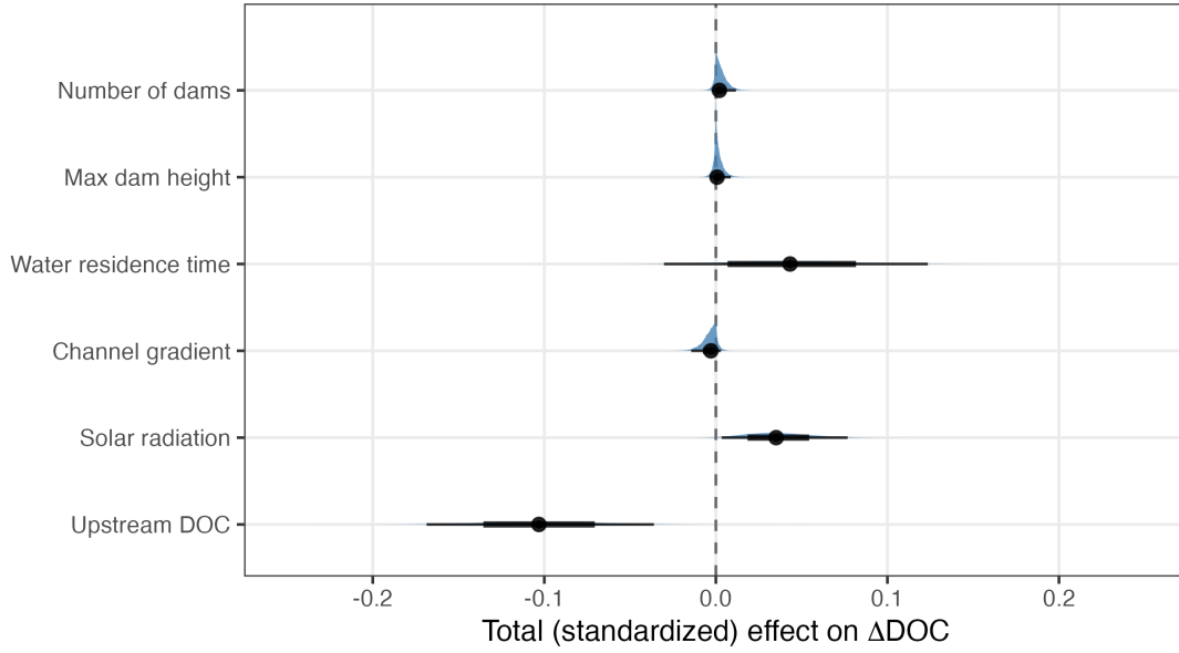
Figure S6: Posterior distributions of the total (standardized) effect of each exogenous driver on \Delta\text{DOC} , obtained by tracing all open causal paths of the SCM. Points: posterior means; thick and thin bars: 66% and 95% credible intervals.
