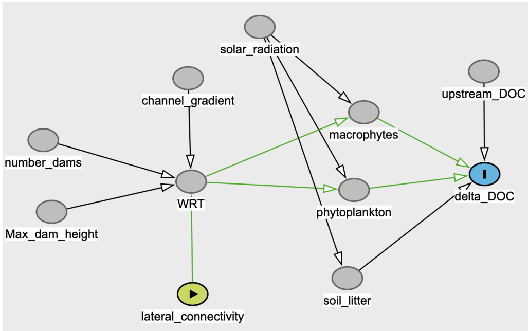
Figure S7: Extended directed acyclic graph (DAG) including lateral stream–wetland connectivity (exposure, green) as a driver of water residence time (WRT). Green edges mark the open front-door paths from connectivity to \Delta DOC (outcome, blue).
