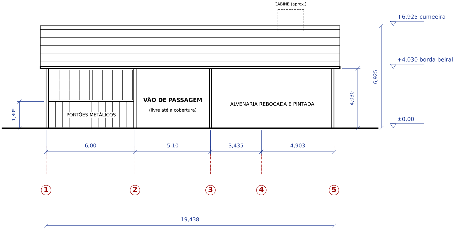
VISTA FRONTAL
