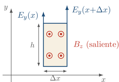
(a) plano xy : Faraday
