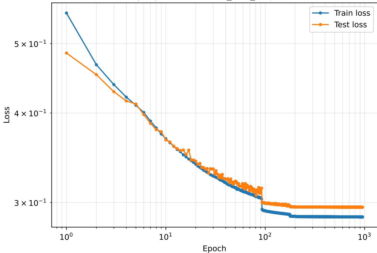
Log-log loss curve: 02_MLP_all-params
