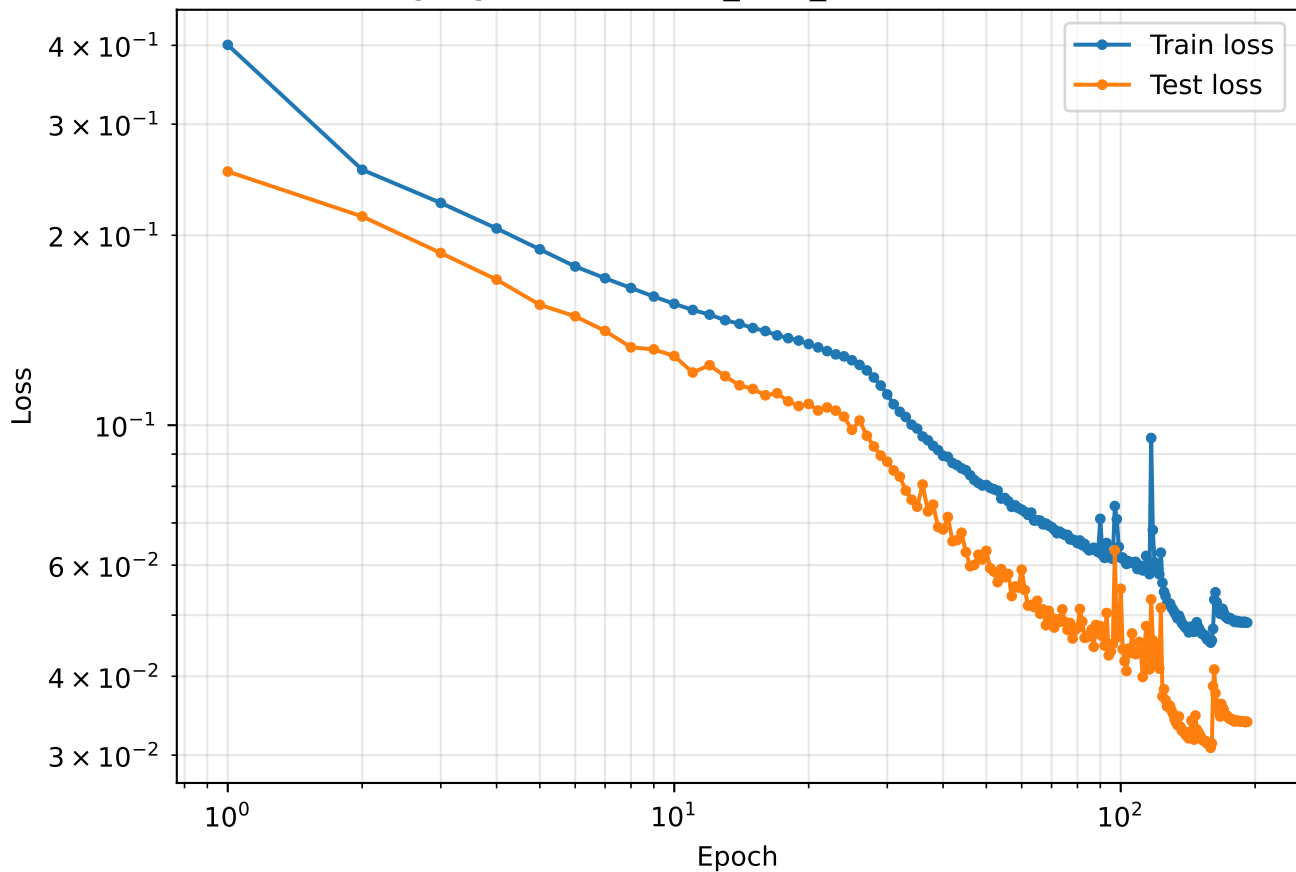
Log-log loss curve: 04_GRU_with-acceleration
