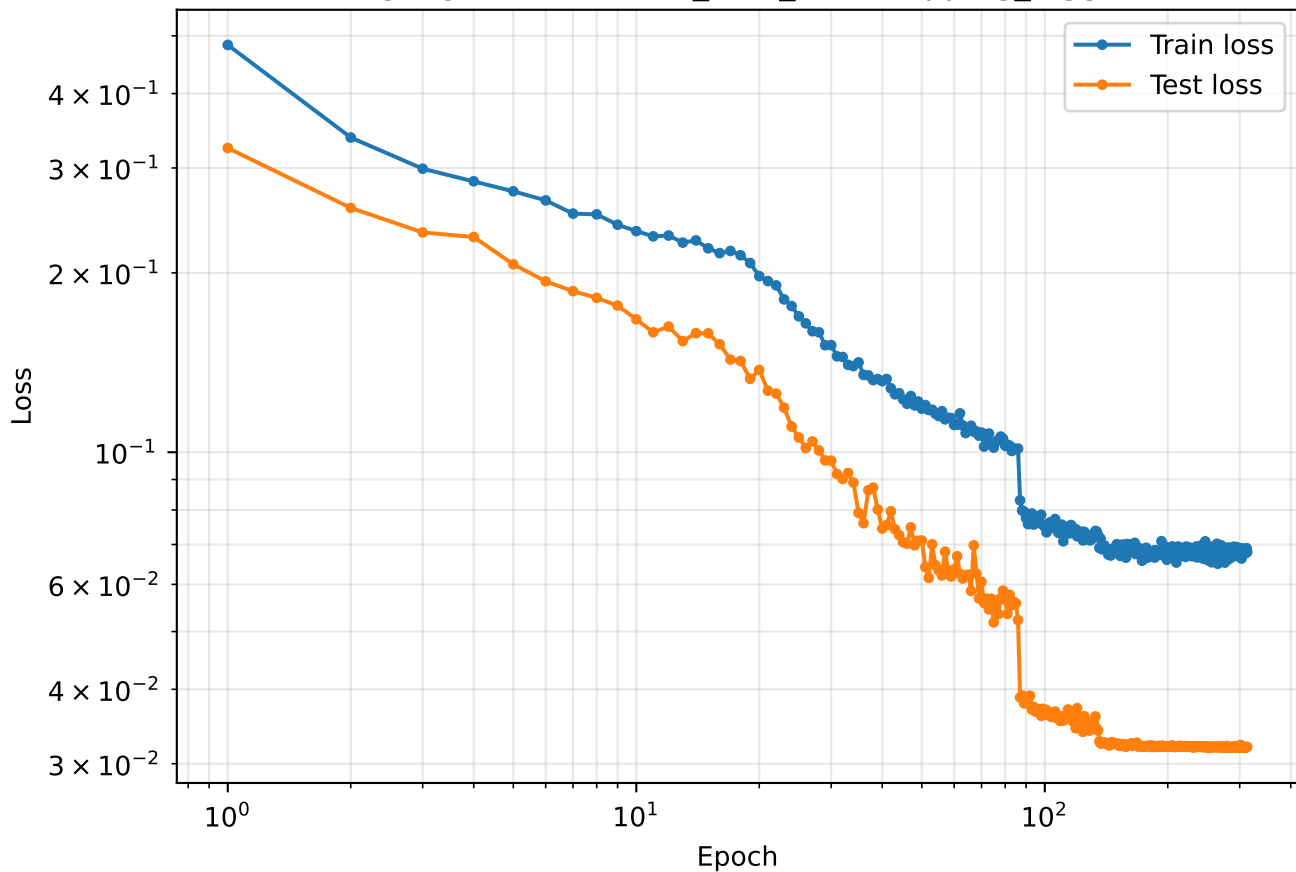
Log-log loss curve: 06_GRU_with-cropping_bigger
