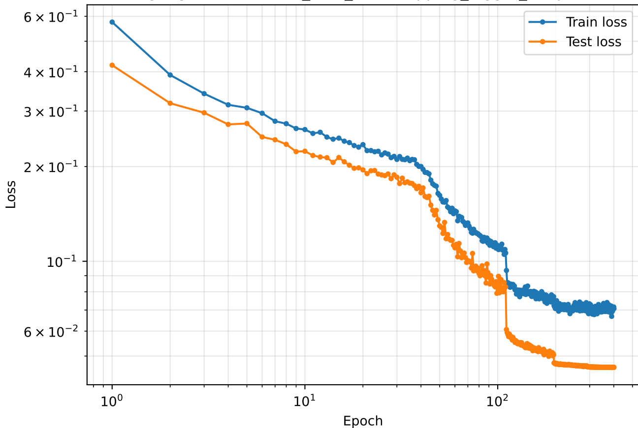
Log-log loss curve: 08_GRU_with-cropping_bigger_endpoint
