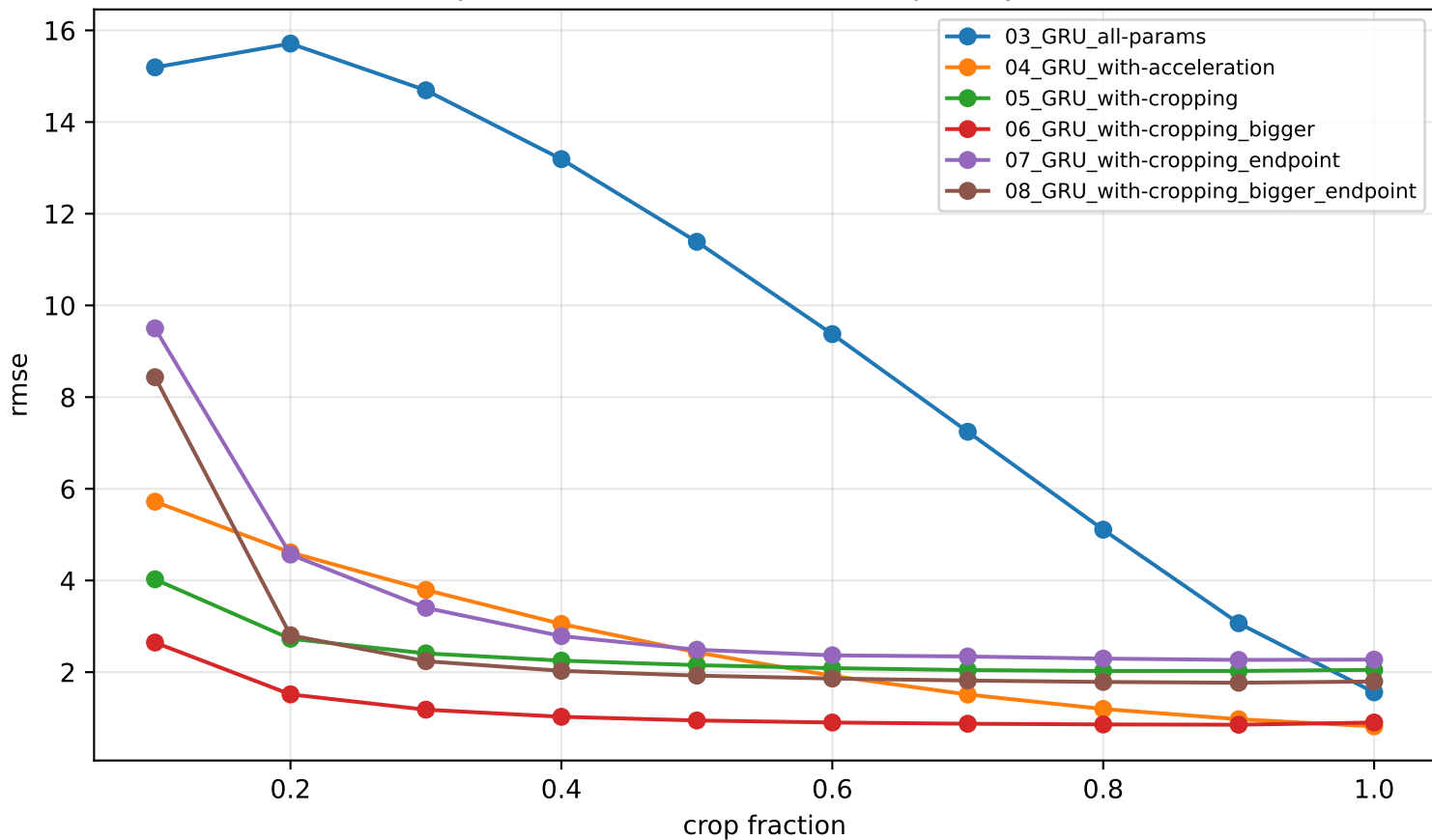
GRU performance vs. observed trajectory fraction
