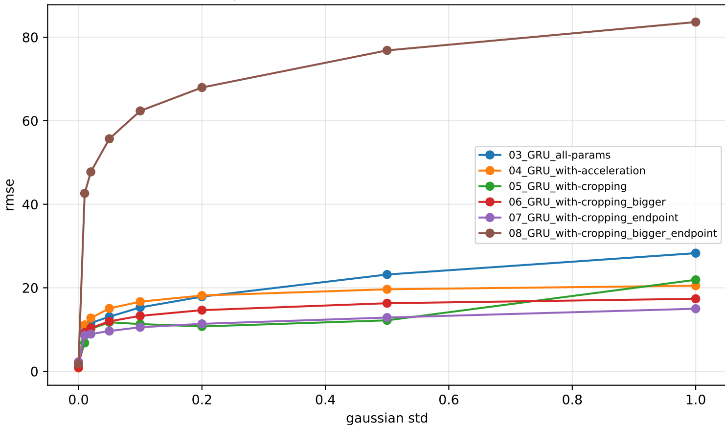
GRU performance vs. Gaussian observation noise
