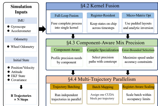
Fig. 4 Compact design overview. The recursive SINS/EKF workload is optimized through whole-scan kernel fusion, component-aware precision specialization, and multi-trajectory parallelism.
