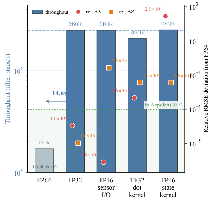
Fig. 3 Precision–performance trade-off over the complete 166,667-step trajectory. Bars report fused-kernel throughput on the left axis; markers report normalized absolute X- and Z-RMSE deviations from fused fp64 on the right axis. Each reduced-precision configuration changes only the named component, with all remaining operations in fp32/IEEE.
