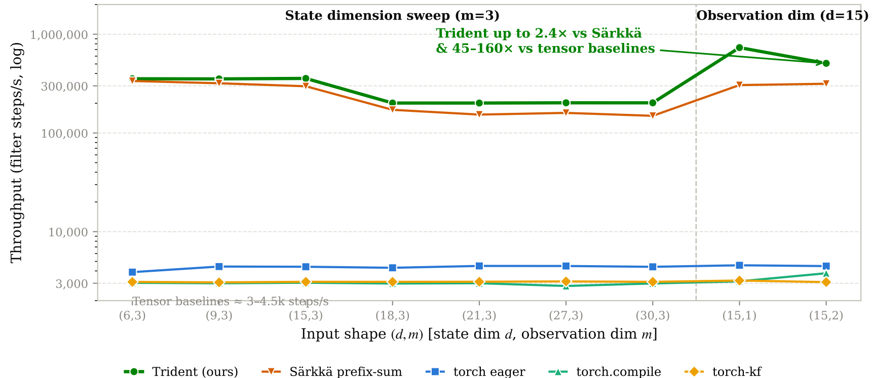
End-to-End Filter Throughput across (d,m) Configurations (NVIDIA H20, N=2000, fp32, B=1)
