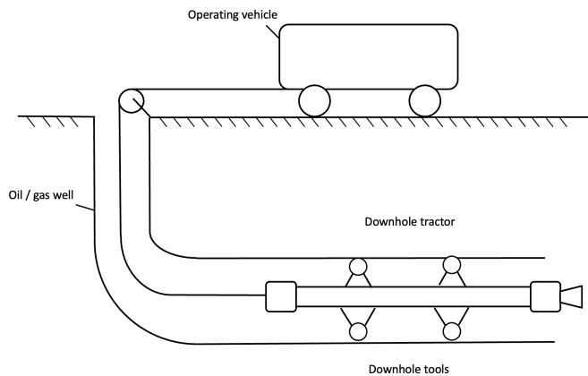
Fig. 1 Schematic of a downhole traction robot conveying a toolstring into the horizontal section of an oil or gas well.
