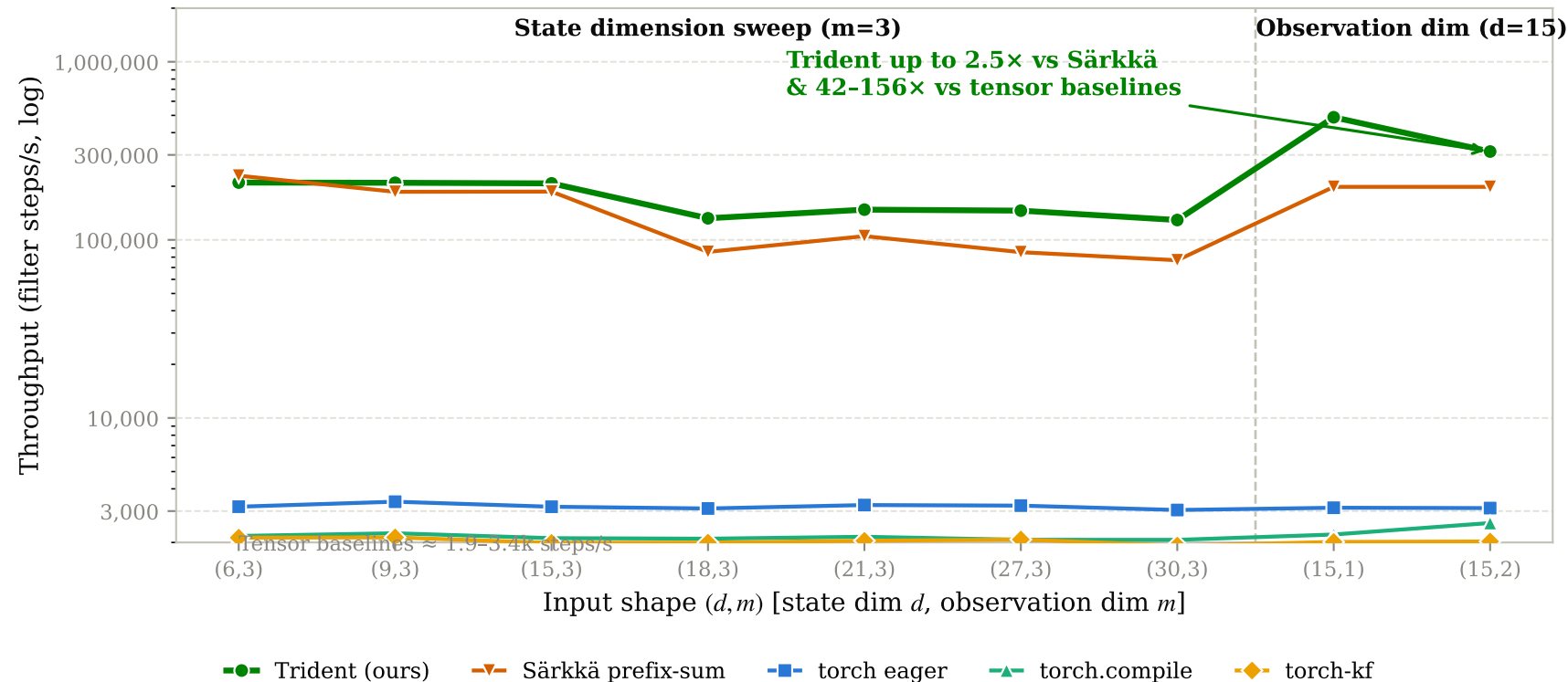
End-to-End Filter Throughput across (d, m) Configurations (NVIDIA A100-SXM4-80GB, N=2000, fp32, B=1)
